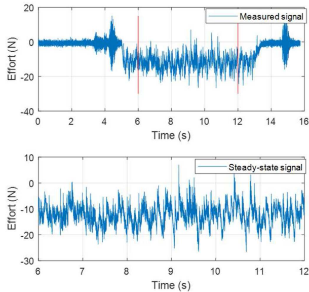
Figure 7: Measured milling force in time domain: (a) total data plot, (b) signal during steady-state phase
