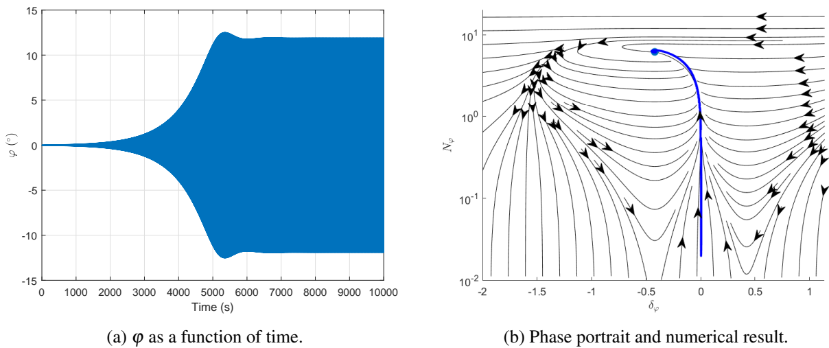
Figure 5 – Case 1: numerical result without NES, N_\varphi(0) = 0.1 \text{ s}^{-1} , \delta_\varphi(0) = 0 \text{ rad}
