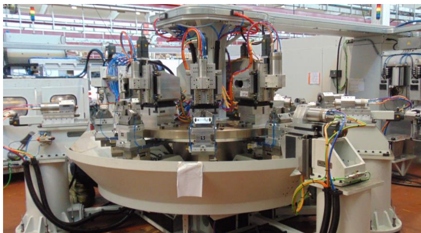
Figure 1: Side view of the analyzed rotary transfer machine
